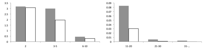
Figure 10: Percentage of queries (y-axis) with their number of out clicks (binned, x-axis) for single-term queries (gray) and multiple term queries (white).
