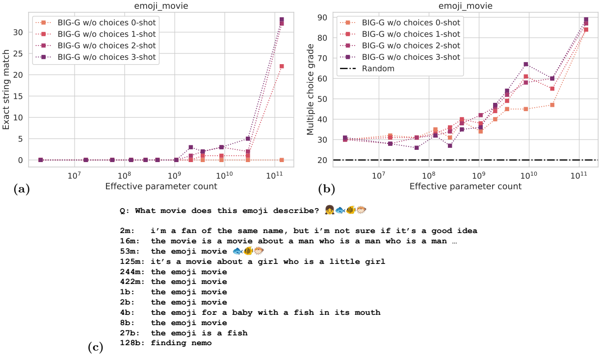
Figure 9: Performance on emoji_movie identification can appear abrupt or gradual depending on the precise task metric. (a) The ability to correctly identify movies seems to appear at a critical scale when measured via exact_string_match . (b) Multiple-choice performance on this task appears to improve more continuously. (c) An example question. The smallest models output irrelevant text, while at intermediate scales models produce output relevant to movies and emojis. The 4B and 27B models identify fish, and the 128B model gives the correct answer. All measurements were performed without the multiple-choice targets appended to the input.
