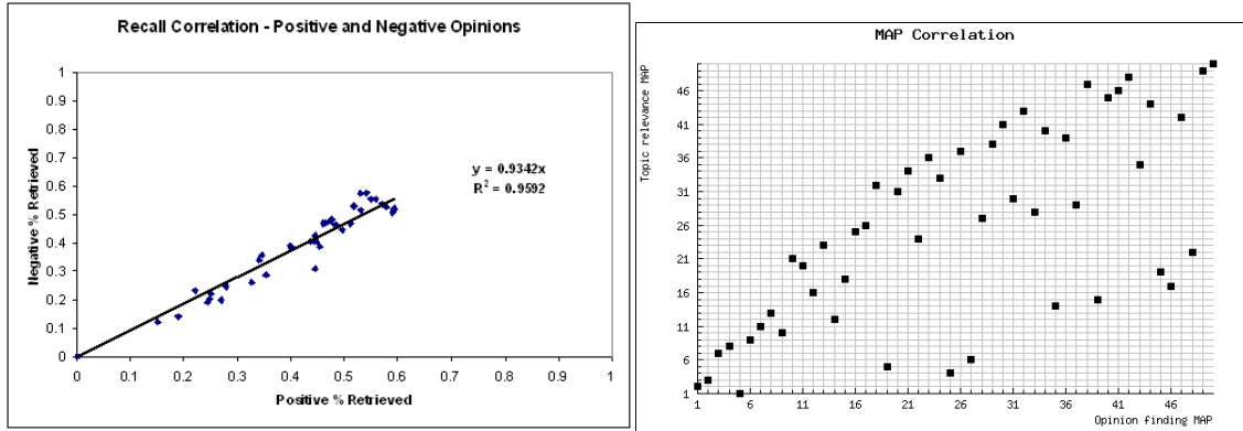
(a) Correlation of positive and negative Recall, by system, over the 57 submitted runs.
