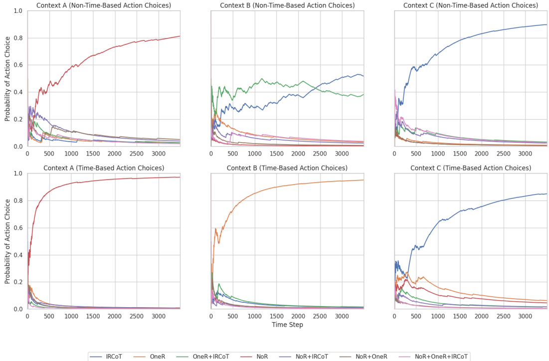
Figure 3: LinUCB action selection distribution for the collaborative action space.
