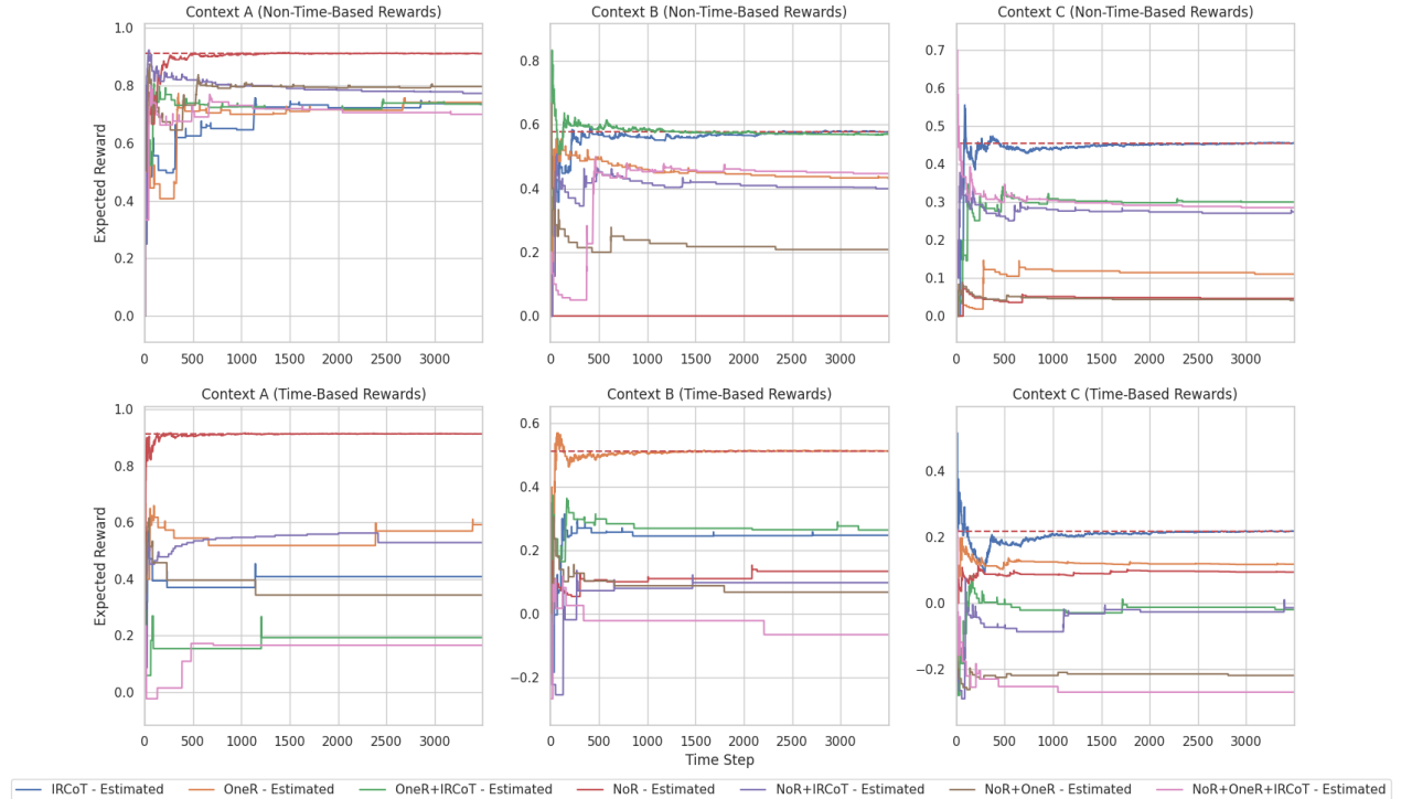
Figure 2: LinUCB expected rewards for the collaborative action space, dashed line depicts real reward for the optimal action.
