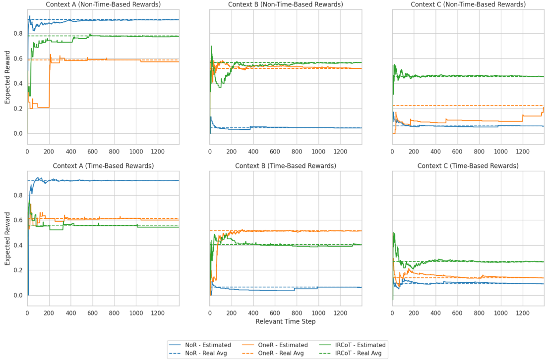
Figure 1: LinUCB expected rewards for individual agents action Space, dashed lines depict the real rewards per action.
