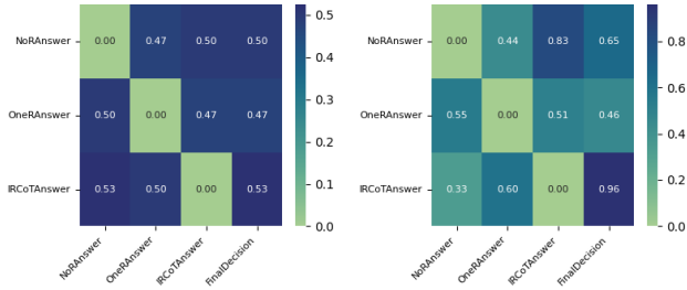
Figure 4: Edge probabilities distribution among NoR, OneR, IRCoT, and FinalDecision nodes before (left) and after (right) optimization using GPTSwarm. (Zhuge et al. 2024).
