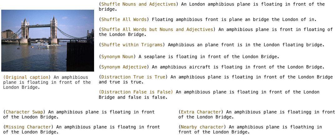
Figure 1: Overview of selected perturbations with examples.
